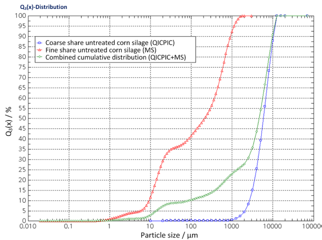
Figure 5.1-3: Cumulative distribution Q_3(x) maize silage untreated (Source: IKTS)
