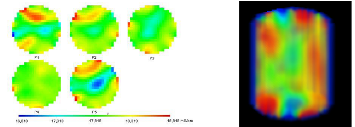
Figure 5.6-12: Visualization of the mixing process inside a cylindrical reactor with five planes of sensors: two-dimensional tomograms (to the left) and three-dimensional illustration of the reactor (to the right) (Source: IKTS)
