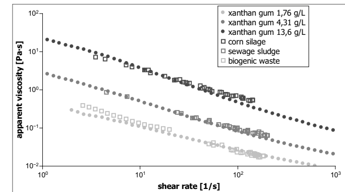
Figure 5.6-3: Comparison of the flow characteristics of substrates and substitute media (Source: BREHMER 2011c)
