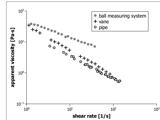
Figure 5.5-7: Comparison of different measurement methods using the example of a substrate mixture of maize silage and coarse rye meal (Source: BREHMER 2011a)
