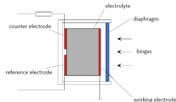
Figure 7.2-3: Schematic representation of an electrochemical cell (Source: Binder GmbH)
