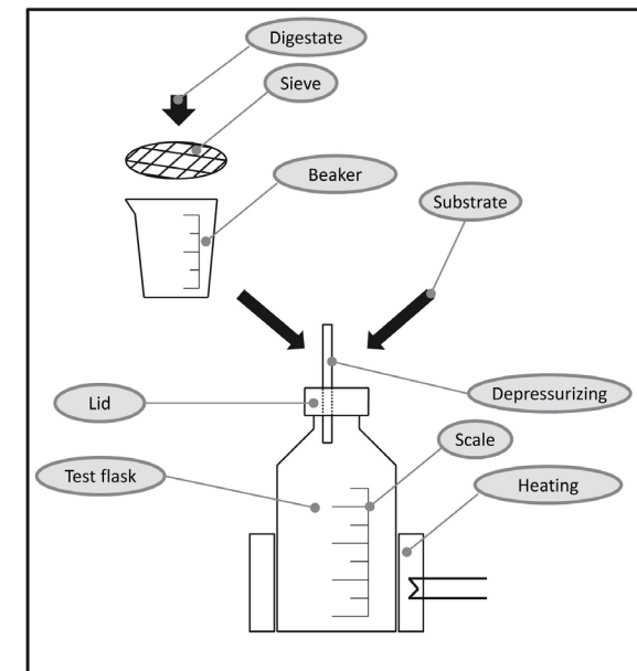
Figure 5.4-2: Test setup with labelling of the individual components (Source: UFZ)
