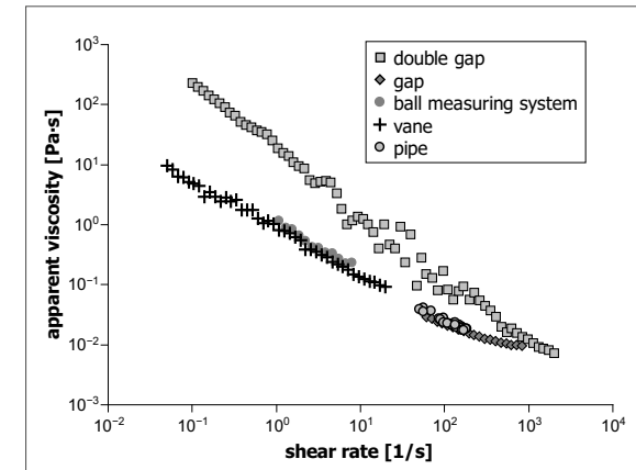
Figure 5.5-4: Comparison of different measurement methods using the example of a substrate mixture of sewage sludge, fats, and biogenous residues (Source: BREHMER 2011a)
