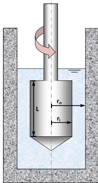
Figure 5.5-1: Cylinder measuring system (Source: BREHMER 2011a)
