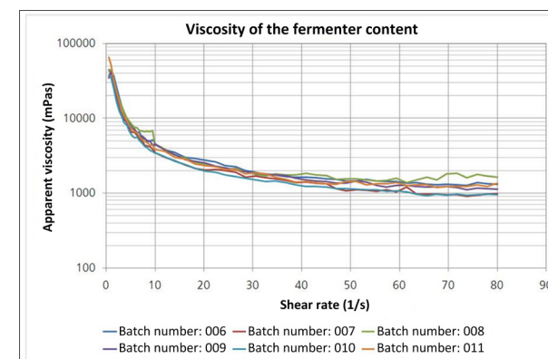
Figure 5.5-12: Viscosity curve of the digester content (Source: IKTS)
