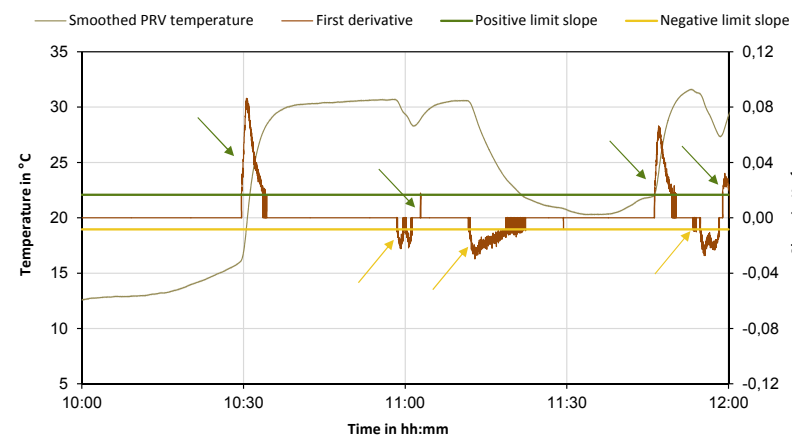
Figure 7.7-2: Calculation of the duration of a triggering event based on temperature data.
