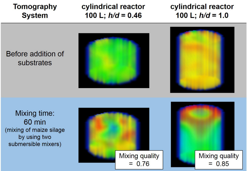
Figure 5.6-13: Average mixing quality in dependence on the reactor geometry (Source: IKTS)
