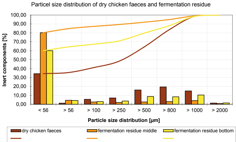
Figure 5.9-3: Depiction of results of sand determination (Source: SCHNEIDER 2010)
