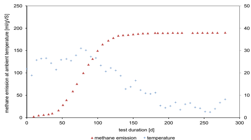
Figure 7.4-5: Methane emission at ambient temperature measured in the storage test stand - Example: sum curve of one test (May - February) with cattle manure on a weekly base (Source: DBFZ)
