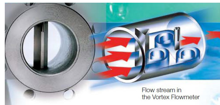
Figure 7.1-1: Principle of vortex method (Source: ABB)
