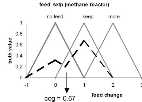
Figure 9.5-3: Fuzzy output variable for feed that gives a defuzzified value of 0.67 (using the center of gravity method)
