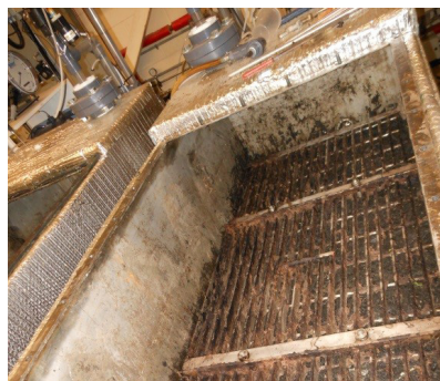
Figure 8.7-3: Pneumatic piston beneath dry digester and grating pulled down onto material to simulate pressure from material height inside the bunker (Source: InnoTech)
