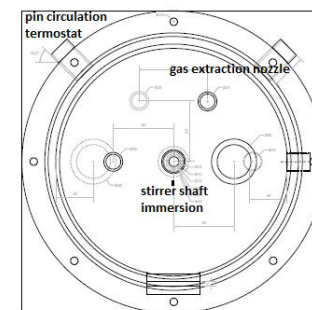
Figure 6.4-1: Technical drawing of a digester with a gross volume of 15 L
