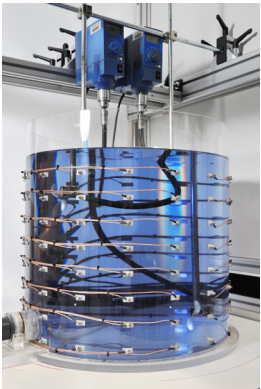
Figure 5.6-9: Process tomography (ITS System P2+) at Fraunhofer IKTS
