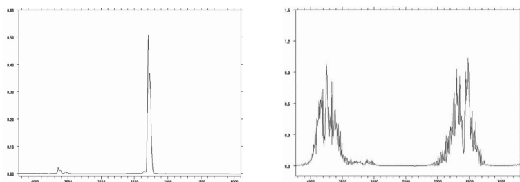
Figure 7.2-1: IR spectra of CO 2 and water vapor (from left to right) (Source: ANSYCO)
