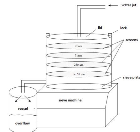
Figure 5.9-1: Setup of sieve machine (Source: SCHNEIDER 2010)
