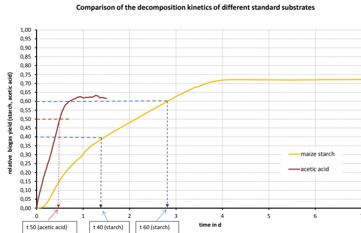
Figure 6.1-1: Typical decomposition kinetics of the standard substrates maize starch and acetic acid and assessment criteria (Source: University of Rostock)
