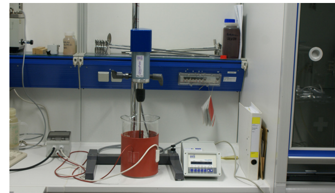
Figure 5.5-15: Test bench for the determination of the apparent viscosity in highly concentrated, fibrous suspensions (Source: IKTS)
