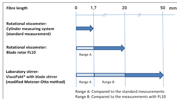
Figure 5.5-10: Measurement method(s) for the determination of the viscosity in dependence on the fibre length (Source: IKTS)
