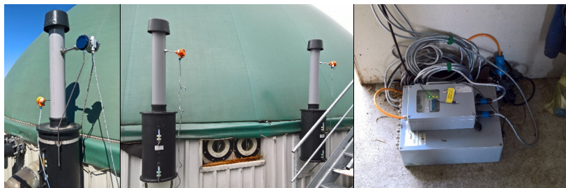
Figure 7.7-3: Exemplary measurement setup at the PRVs of an agricultural biogas plant; Left: Flow velocity and temperature sensor installed at the PRV of the main digester (cp. Fig. 5.7-1); Centre: Temperature sensors installed at PRVs of the gastight covered digestate storage; Right: Data logger; Figure modified from (LIEBETRAU et al. 2017)
