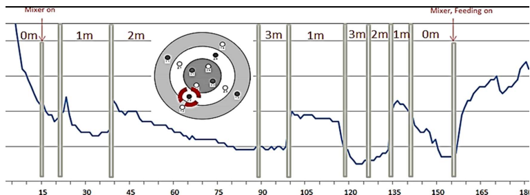
Figure 10.2-4: Investigation of redox potential gradients with the miniaturised sensor device in a 920 m³ biogas digester (KIELHORN et. al 2015)
