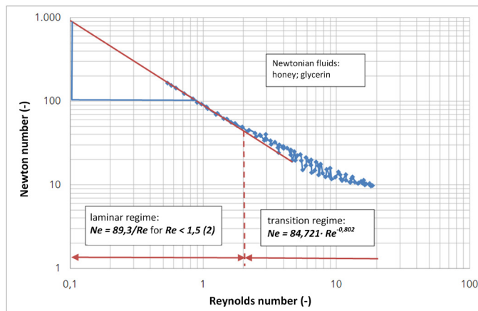
Figure 5.5-16: Performance characteristics of the stirrer system utilised for the viscosity measurement (Source: IKTS)
