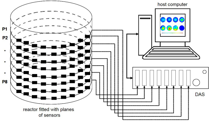
Figure 5.6-10: Components of the ERT system at Fraunhofer IKTS by means of the example of a cylindrical reactor with a height to diameter ratio of 1 and eight sensor planes.
