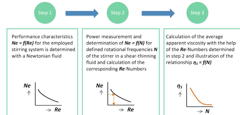
Figure 5.5-14: Approach for the determination of the viscosity according to METZNER & OTTO
