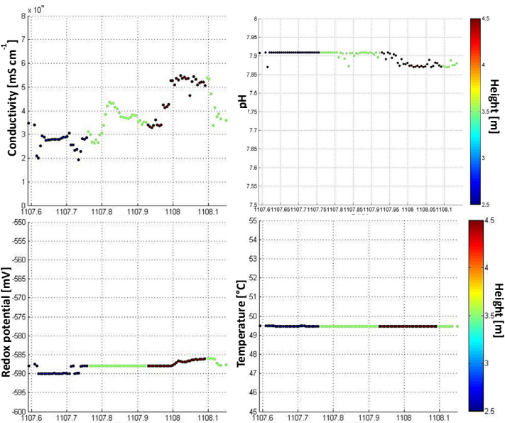
Figure 10.2-5: Investigation of conductivity, redox potential, pH-value, and temperature gradients with commercial sensors in a 920 m³ biogas digester (KIELHORN et. al 2015).
