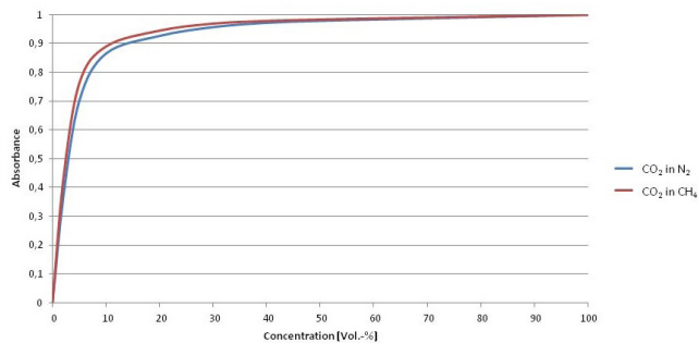
Figure 10.4-4: Concentration-dependent infrared absorption of carbon dioxide at 4.3 \mu\text{m} with background gas nitrogen or methane
