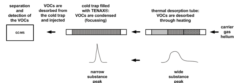
Figure 7.8-2: Schematic depiction of the thermal desorption with subsequent analysis (Source: Fraunhofer UMSICHT)
