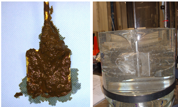
Figure 5.5-19: Wrapping around blade stirrer and vortex formation (Source: IKTS)
