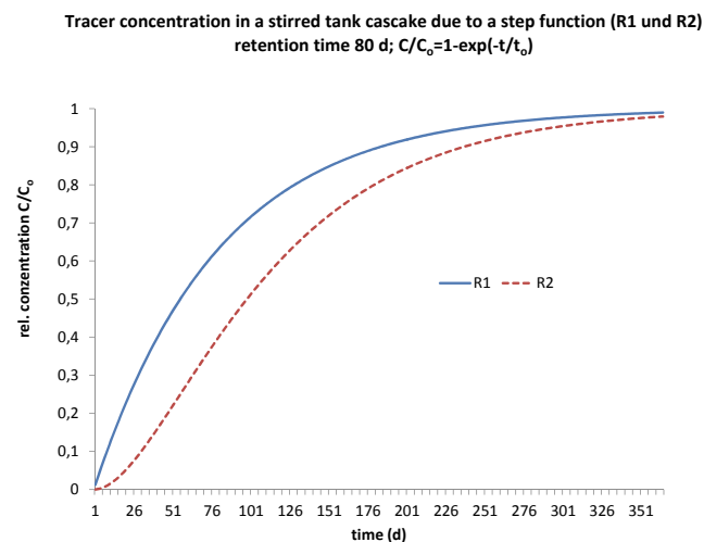
Figure 6.4-3: Tracer concentration in a stirred tank cascade due to a step function in the case of a retention time of 80 d (Source: DBFZ)
