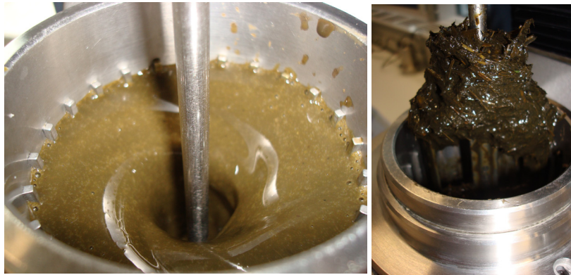
Figure 5.5-13: Faulty measurements due to vortex formation and wrapping around a stirrer shaft (Source: IKTS)
