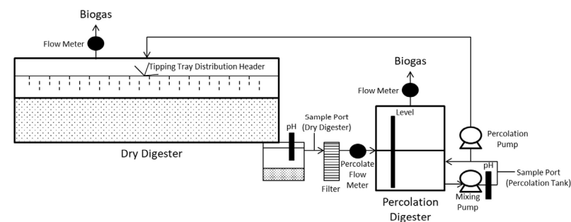
Figure 8.7-2: Overall process schematic (Source: InnoTech)
