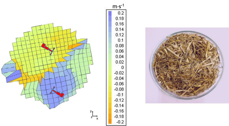
Figure 5.6-14: Velocity profile (to the left) of a suspension consist of xanthan gum and wheat straw (to the right) by using two submersible mixers (Source: IKTS)
