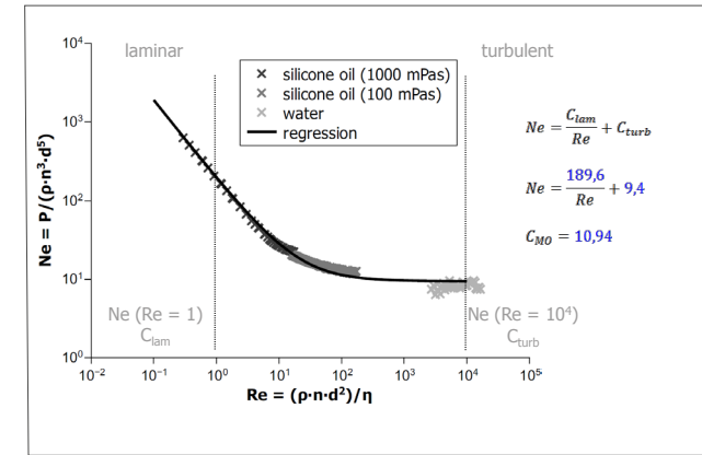
Figure 5.5-5: Example for the functional dependency of the power input on the Reynolds number for a vane (Source: BREHMER 2011b)
