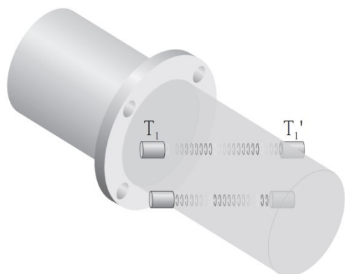
Figure 7.1-2: Principle of ultrasonic method (Source: Endress & Hauser)
