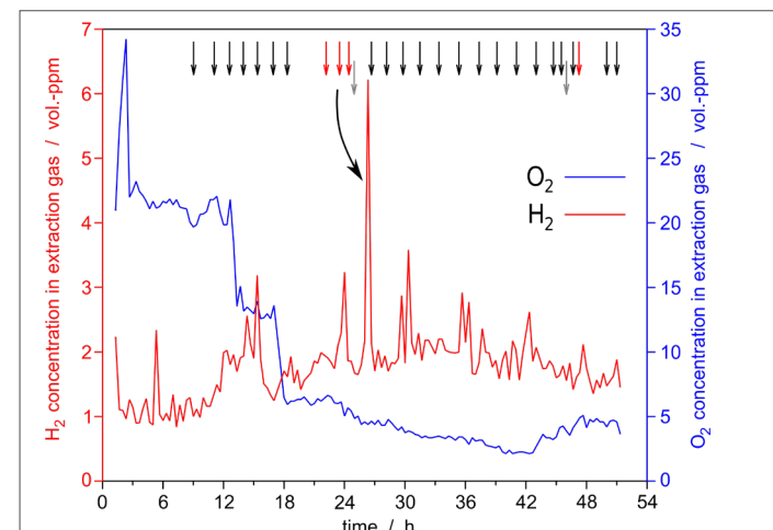
Figure 10.1-3: Online measurement of the dissolved hydrogen and the dissolved oxygen in a biogas plant, feeding times marked with arrows, red = solid cattle dung, black = maize silage, grey = cattle manure (Source: KSI)
