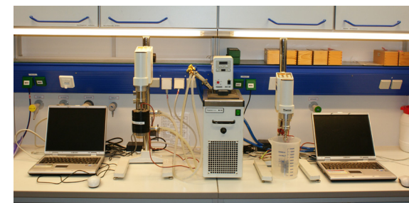
Figure 5.5-11: ViscoTester 550 with cylinder measuring device (left) and with blade stirrer FL10 (right) for the measurement of fermentation substrates (Source: IKTS)
