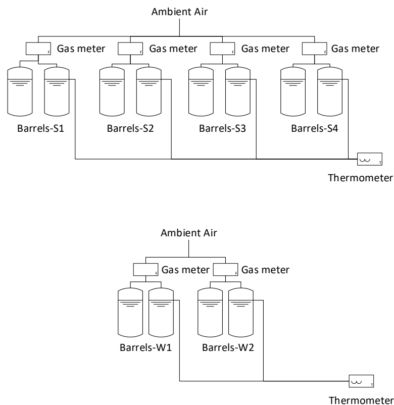
Figure 7.4-1: Piping and Instrumentation Diagram of the manure storage test stand (Source: DBFZ Masula)
