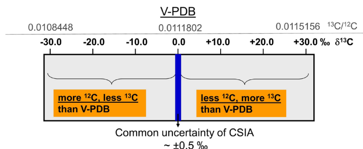
Figure 6.7-2: Illustration of the delta scale for stable carbon isotope ratios ( ^{13}\text{C}/^{12}\text{C} ) as an excerpt ranging from -30 to +30 ‰. The anchor of the \delta^{13}\text{C} -scale is V-PDB (Vienna-Pee Dee Belemnite, ^{13}\text{C}/^{12}\text{C} = 0.0111802 ). CSIA – Compound-specific stable isotope analysis
