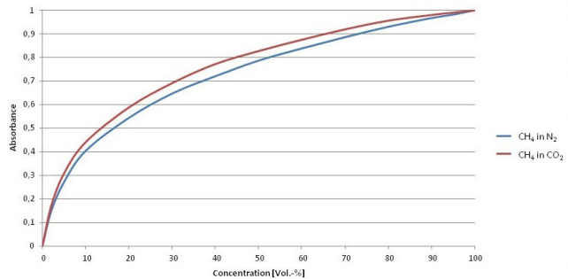
Figure 10.4-3: Concentration-dependent infrared absorption of methane at 3.4 \mu\text{m} with background gas nitrogen or carbon dioxide
