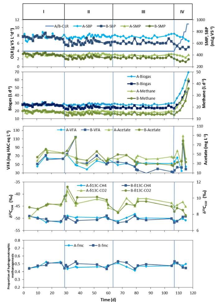
Figure 6.7-10: Organic loading rate (OLR), biogas and methane production, concentration of volatile fatty acids (VFA) and acetate, \delta^{13}\text{C}_{\text{CH}_4} - and \delta^{13}\text{C}_{\text{CO}_2} -values as well as proportion of hydrogenotrophic methanogenesis derived from carbon isotope data for a long-term experiment with two biogas reactors (A, B) using DGGs as biogas substrate operated with varying feeding regimes:
