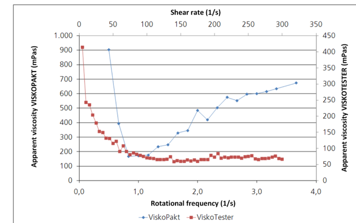
Figure 5.5-18: Faulty assessment of the viscosity for low-viscous material systems in the case of utilisation of the ViscoPakt®-laboratory stirrer (Source: IKTS)
