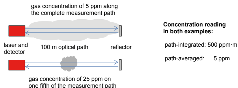
Figure 7.6-2: Schematic depiction of path-integrated and path-averaged concentration information (Source: DBFZ)
