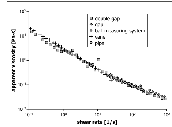
Figure 5.5-3: Comparison of different measurement methods using the example of sewage sludge (Source: BREHMER 2011a)
