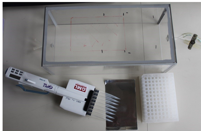
Figure 6.6-1: Multi-channel pipettor, aluminium foil, 96-well plate, and an example for a simple chamber with gas ports for flushing with nitrogen. By simply moving up the box during pipetting, excessive sample contact with oxygen is avoided. When dilution series is completed, the 96-well plate is sealed with the aluminium foil under the nitrogen stream
