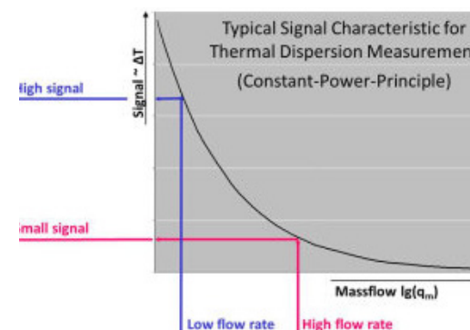
Figure 7.1-4: Signal level of thermal mass flow meter depending on gas flow rate (Source: Binder GmbH)
