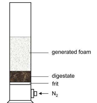
Figure 5.3-2: Scheme of the foam generator for the determination of the foaming potential of a liquid mixture (Source: UFZ)
