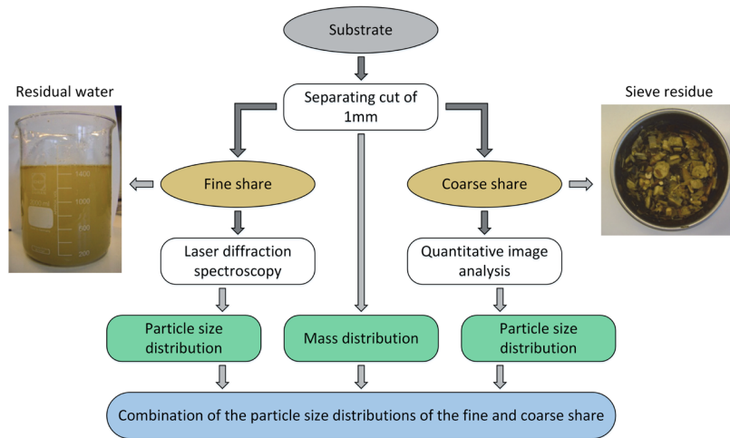
Figure 5.1-1: Principle of granulometric assessment (Source: IKTS)
