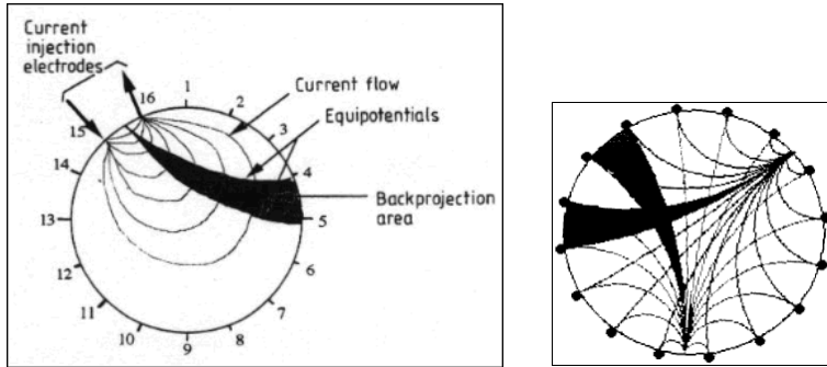
Figure 5.6-11: Measuring principle of the ERT system (Source: according to LEE 2009)
