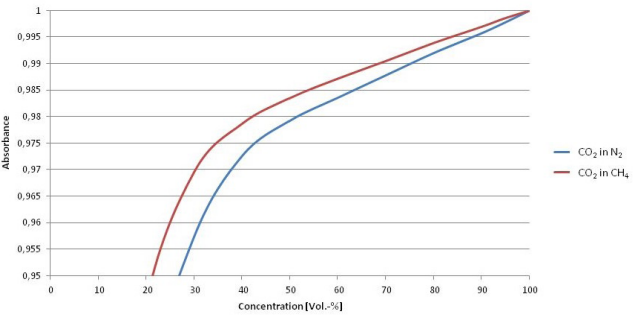
Figure 10.4-5: Concentration-dependent infrared absorption of carbon dioxide at 4.3 \mu\text{m} with background gas nitrogen or methane (high range)
