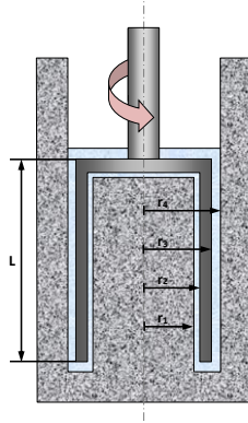
Figure 5.5-2: Double slit measuring system (Source: BREHMER 2011b)
