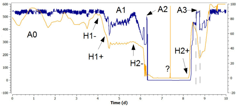
Figure 9.5-4: CHP power (left y-axis; A, dark (blue)) vs. gas storage level (right y-axis, H, orange). A0: CHP runs with full power, A1: reduced power, A2 and A3: see text.; H1-, H2-: stop of substrate dosage; H1+, H2+: restart of substrate dosage
