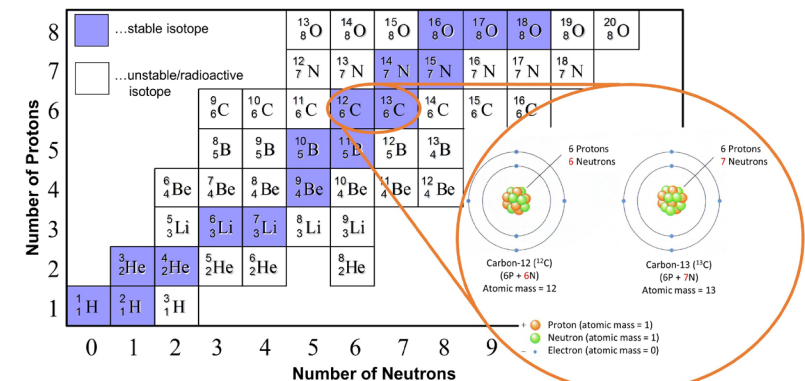
Figure 6.7-1: Overview on isotopes of chemical elements ranging from hydrogen to oxygen. The enlarged excerpt shows a simple atomic model of the two stable carbon isotopes with the derivation of their atomic masses based on the different numbers of neutrons. P – protons, N – neutrons
