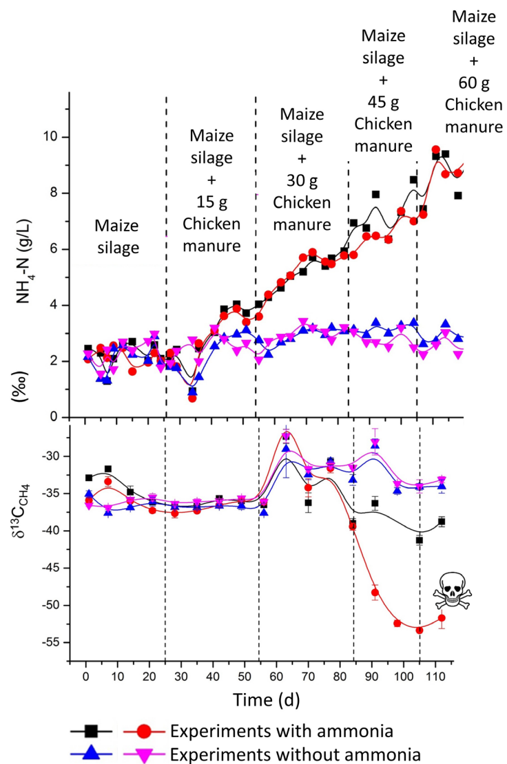
Figure 6.7-9: Changes in \delta^{13}\text{C}_{\text{CH}_4} -values due to the inhibition of biogas production caused by increasing ammonium concentration ( \text{NH}_4\text{-N} ). Modified from Lv et al. (2014)
