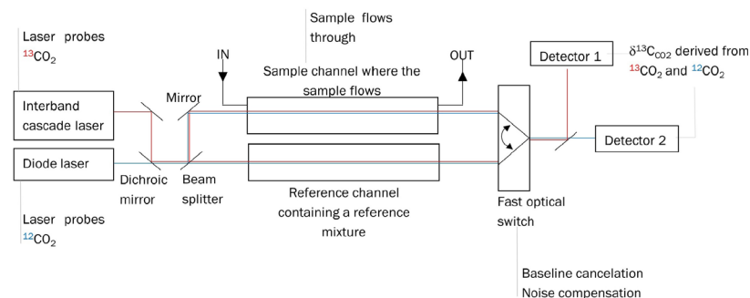
Figure 6.7-4: Scheme of an example of an IRIS system for CSIA of \text{CO}_2
