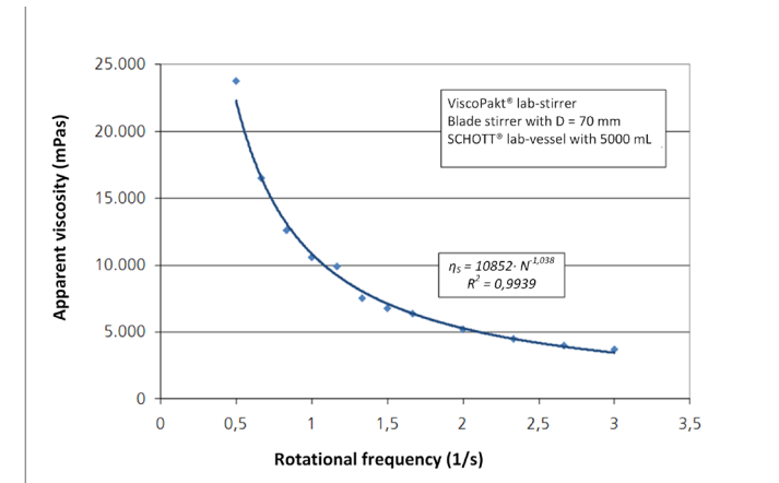
Figure 5.5-17: Apparent viscosity in dependence on the rotational frequency for the hydrolysate of a biogas plant (Source: IKTS)
