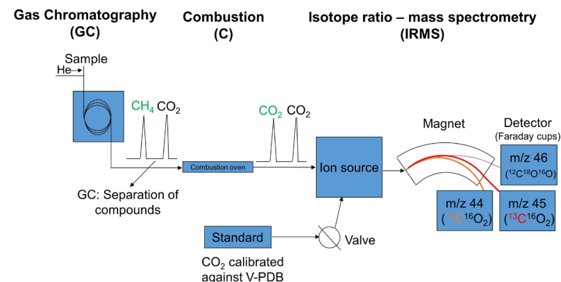
Figure 6.7-3: Scheme of gas chromatography - combustion - isotope ratio mass spectrometry (GC-C-IRMS) for CSIA of carbon for \text{CH}_4 and \text{CO}_2
