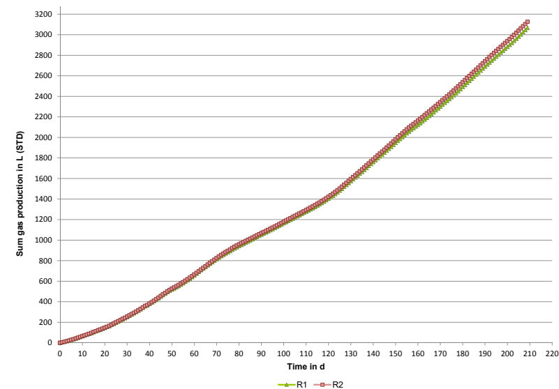
Figure 6.4-5: Cumulated gas production of two digesters in parallel operation (Source: DBFZ)
