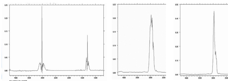
Figure 7.2-2: IR spectra of methane, ethane and propane (from left to right) (Source: ANSYCO)
