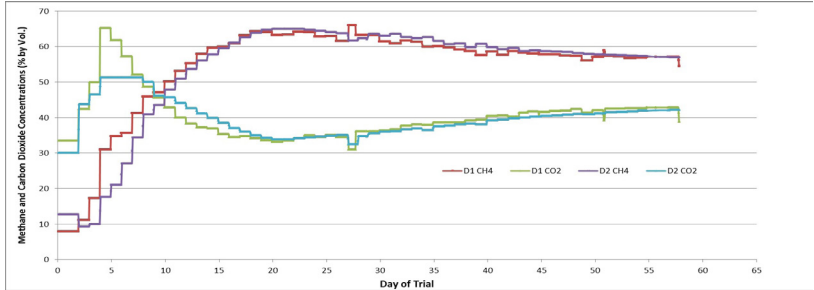
Figure 8.7-10: Biogas compositional data from Digester 1 and 2 throughout the trial (Source: InnoTech)
