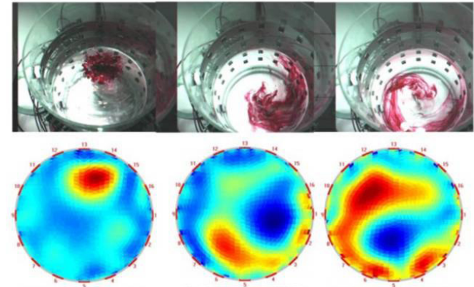
Figure 5.6-8: Visual comparison of the mixing of two liquids using ERT (Source: ITS 2012)
