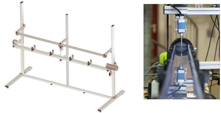
Figure 6.6-6: Towing-channel for the calibration and determination of the constants of a film sensor
