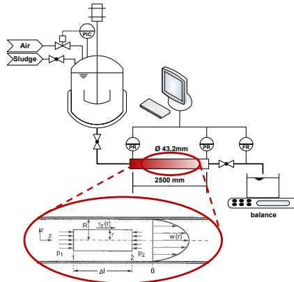
Figure 5.5-9: Flow diagram for the laminar flow tube (Source: BREHMER 2011a; KRAUME 2004)
