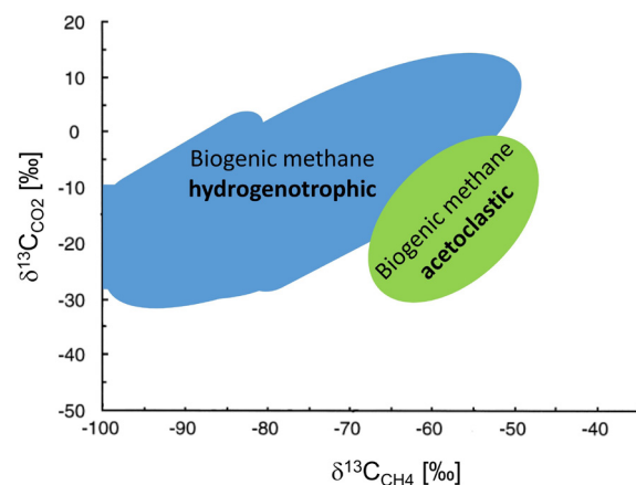
Figure 6.7-7: Differentiation of methanogenic pathways using the comparison of \delta^{13}\text{C}_{\text{CH}_4} - and \delta^{13}\text{C}_{\text{CO}_2} -values. Modified from WHITICAR (1999)
