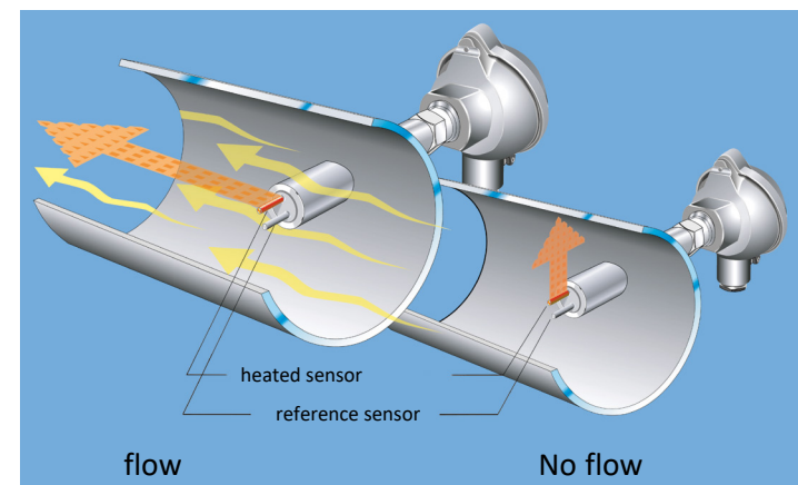
Figure 7.1-3: Principle of thermal dispersion method (Source: Binder GmbH)
